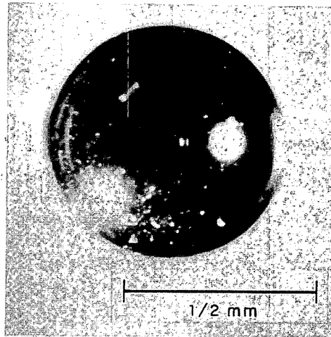
Fig. 2. An active fallout particle from a tower shot in Nevada. The particle is spherical with a brilliant, glossy surface.
